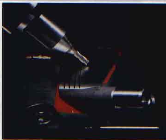
The unique Accuform computer-controlled cutter cuts V-grooves into an Accuform iron.
